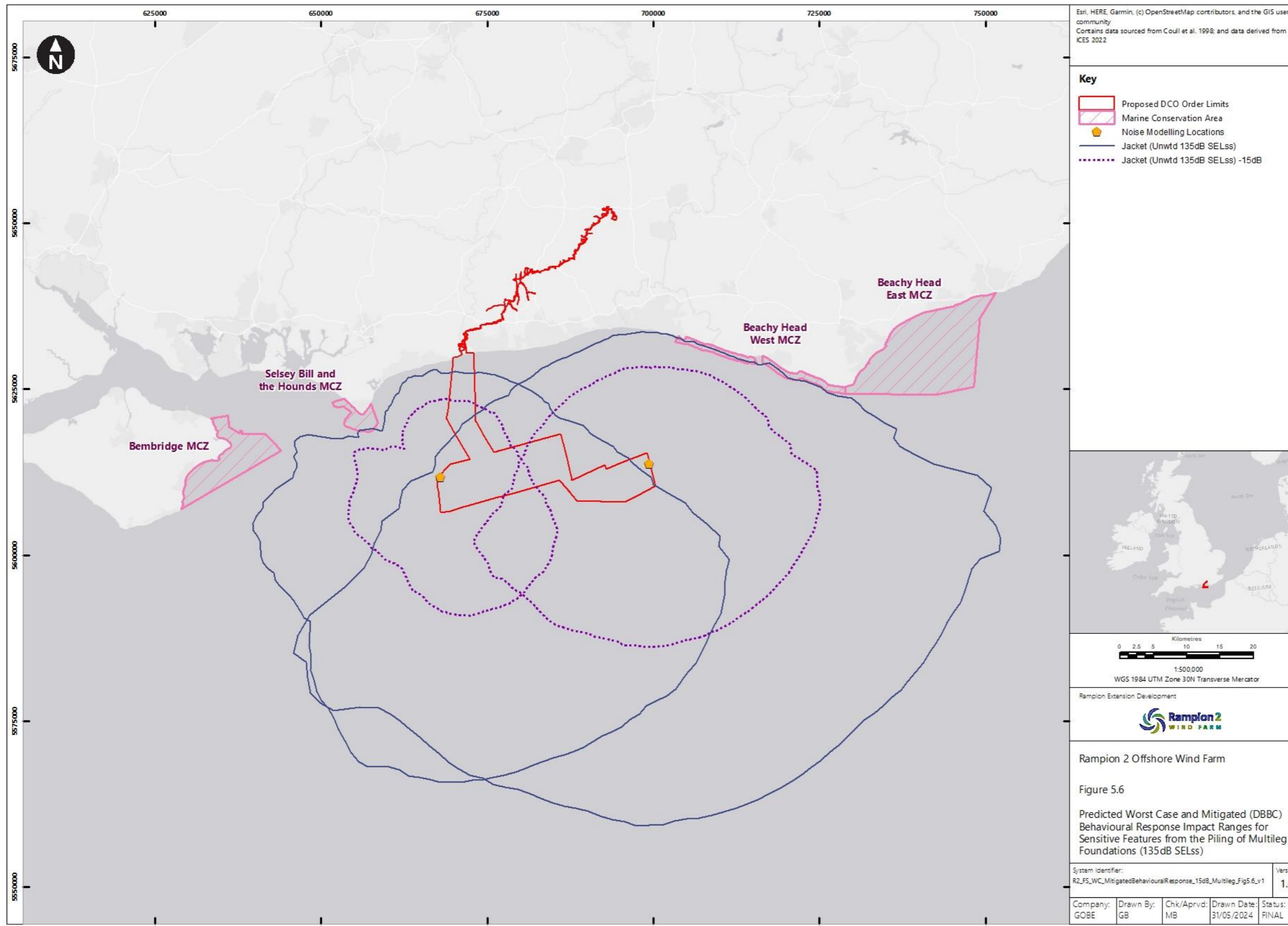
Figure 5-6 Predicted Worst Case and Mitigated (DBBC) Behavioural Response Impact ranges for Sensitive Features from the Piling of Multileg Foundations (135dB SELss)
